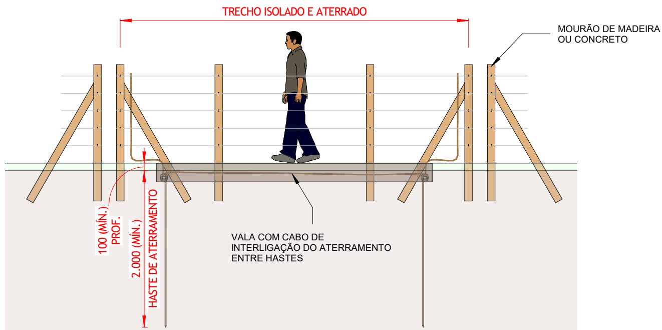
VISTA FRONTAL
