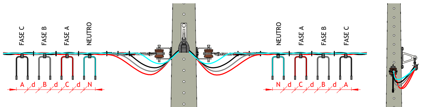
VISTA FRONTAL
