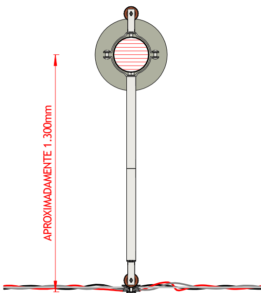
VISTA FRONTAL
