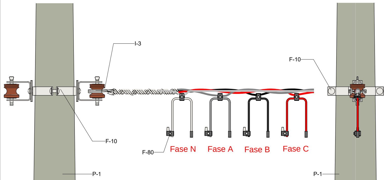
VISTA FRONTAL
