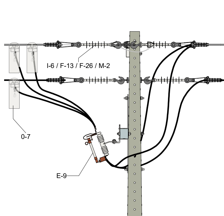
VISTA FRONTAL
