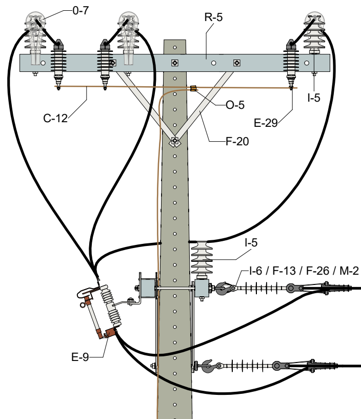
VISTA FRONTAL
