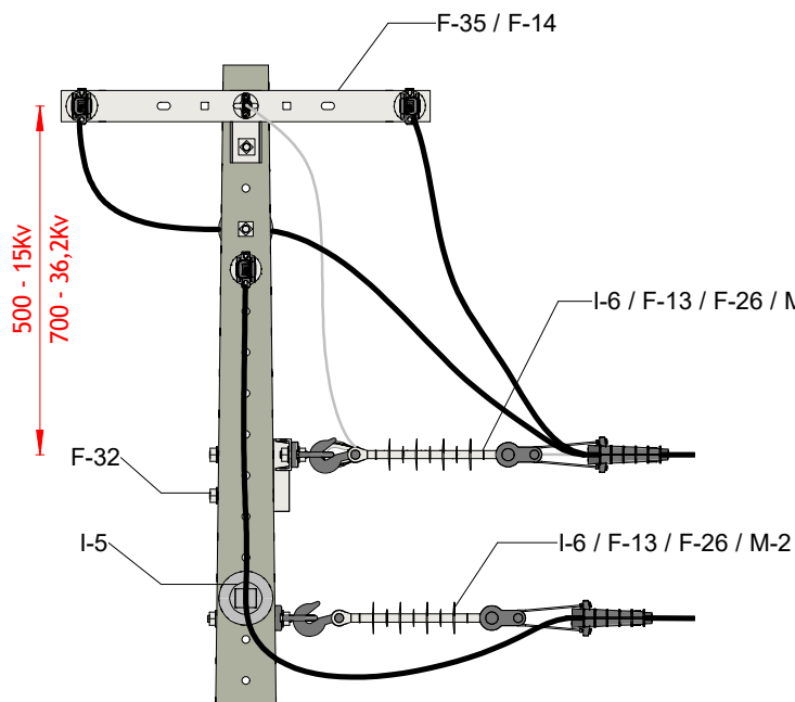
VISTA FRONTAL
