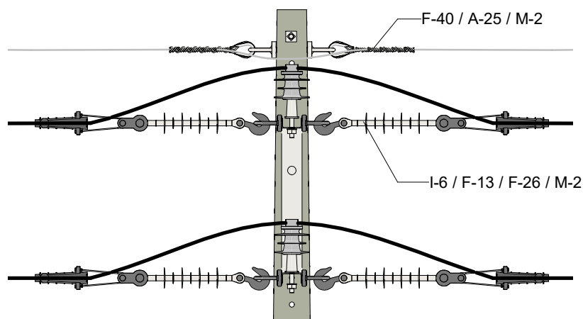
VISTA FRONTAL
