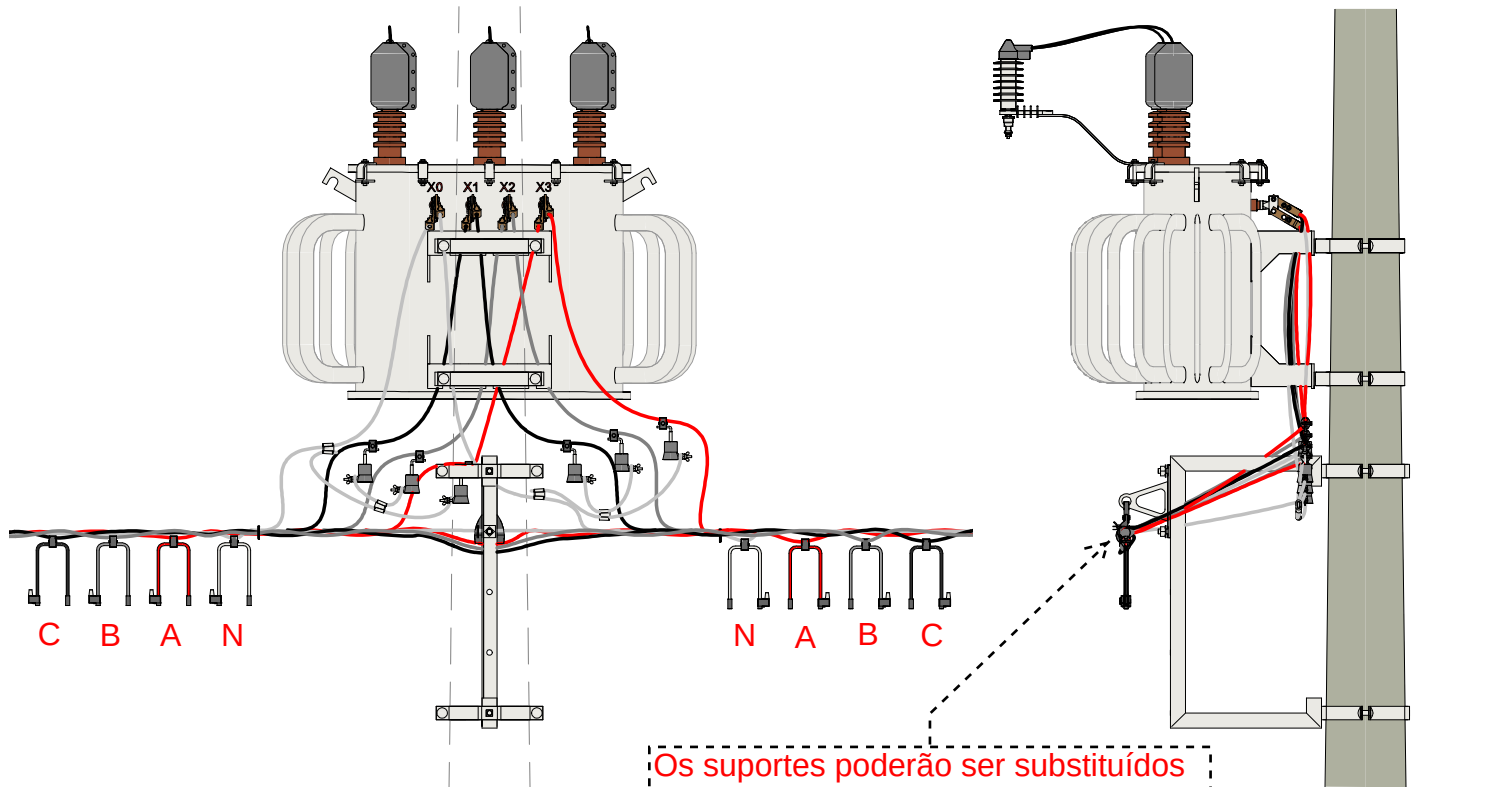
VISTA FRONTAL
