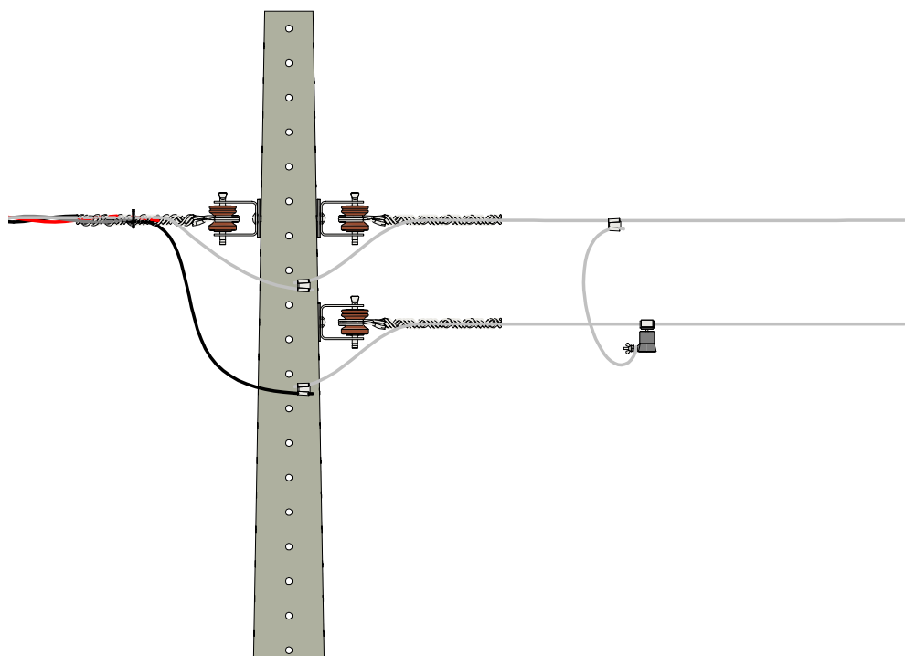
VISTA FRONTAL
