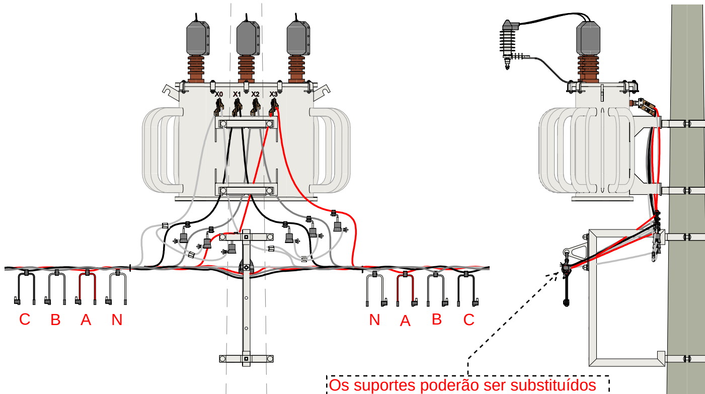
VISTA FRONTAL
