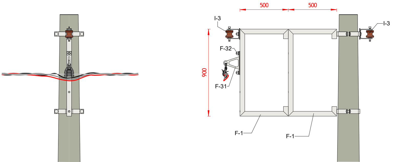
VISTA FRONTAL
