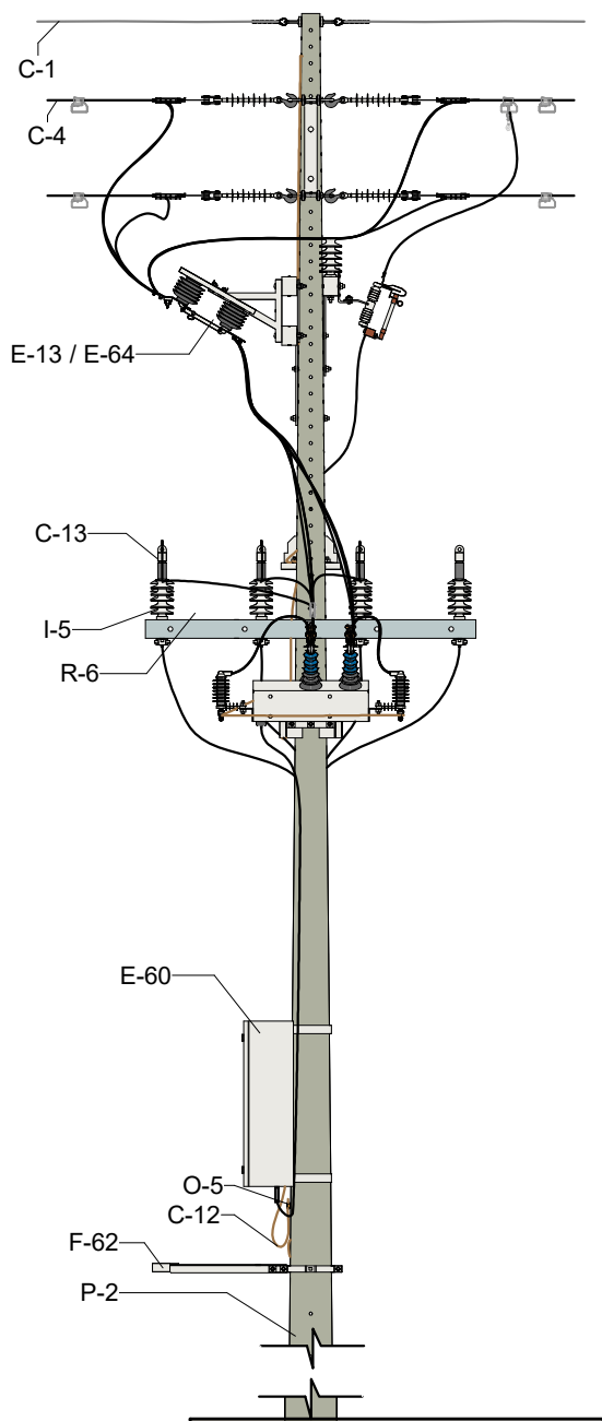
VISTA FRONTAL
