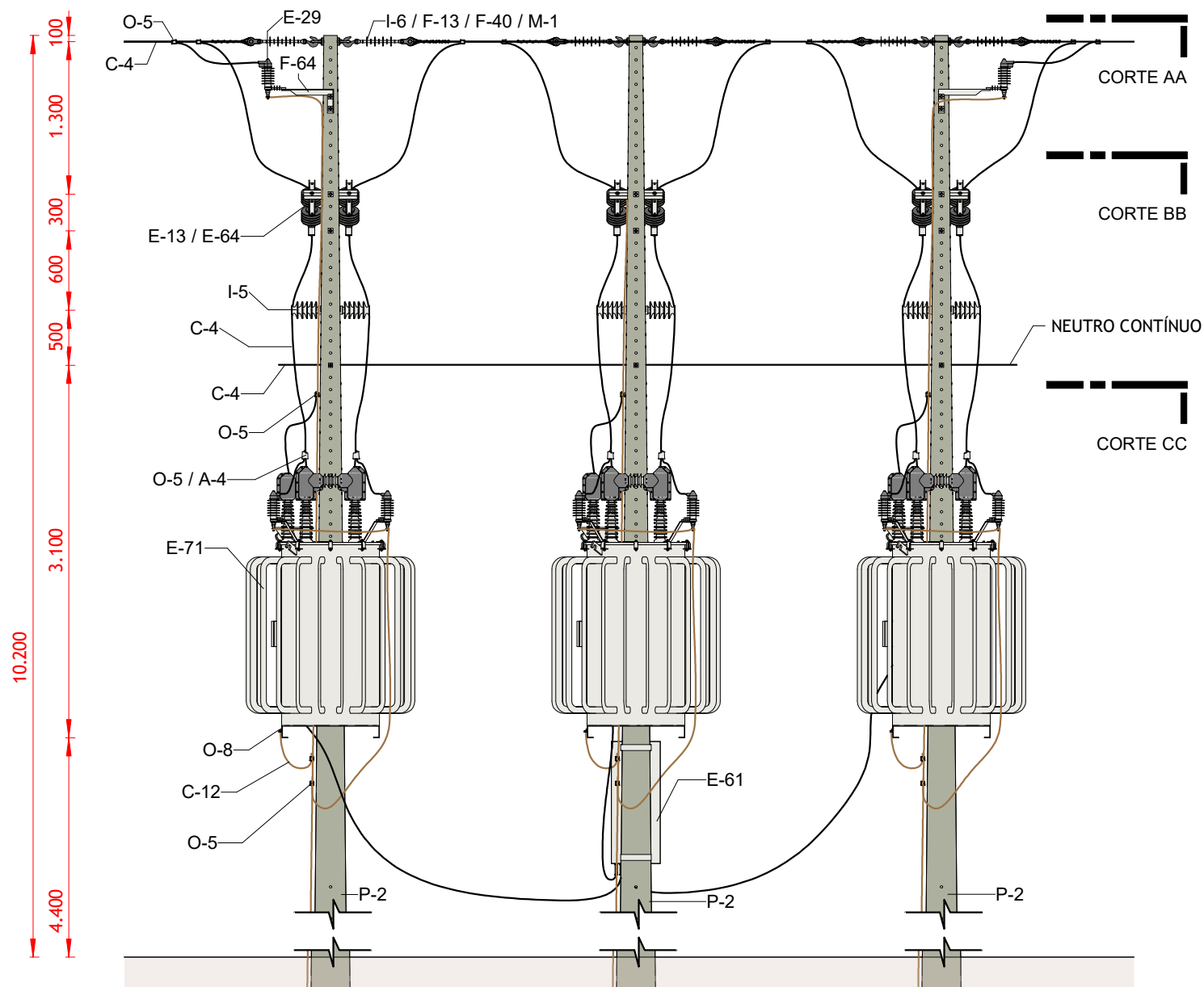
VISTA FRONTAL
