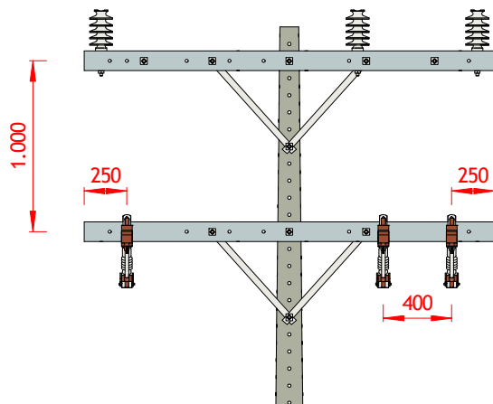
VISTA FRONTAL
