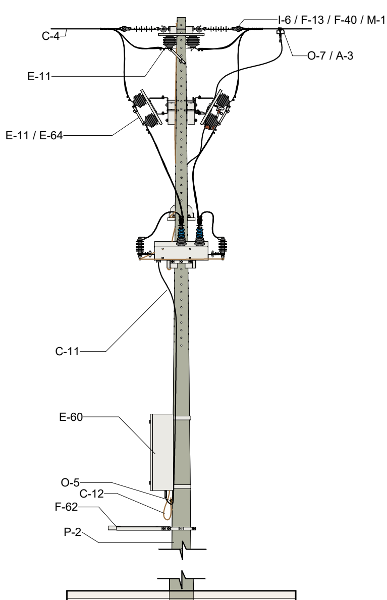
VISTA FRONTAL
