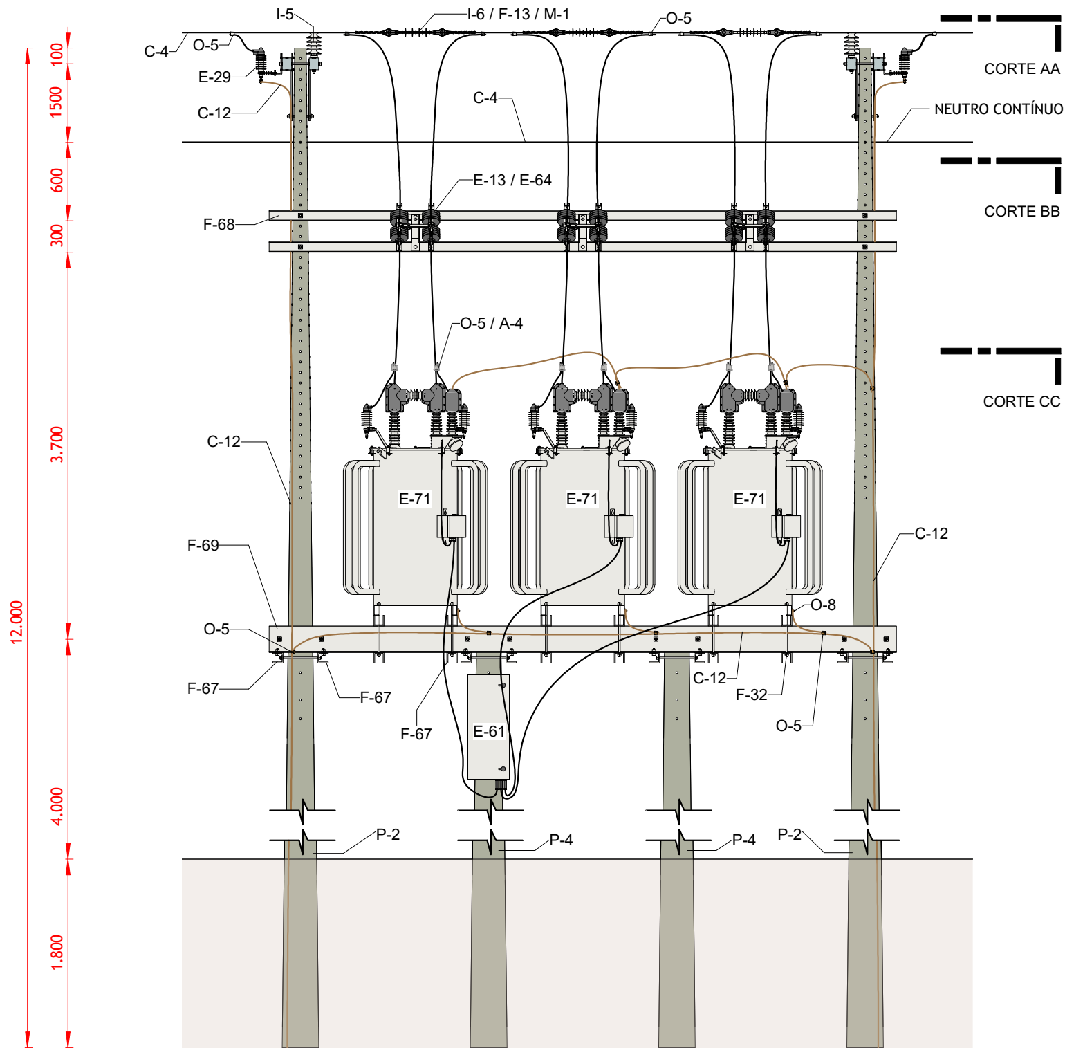
VISTA FRONTAL
