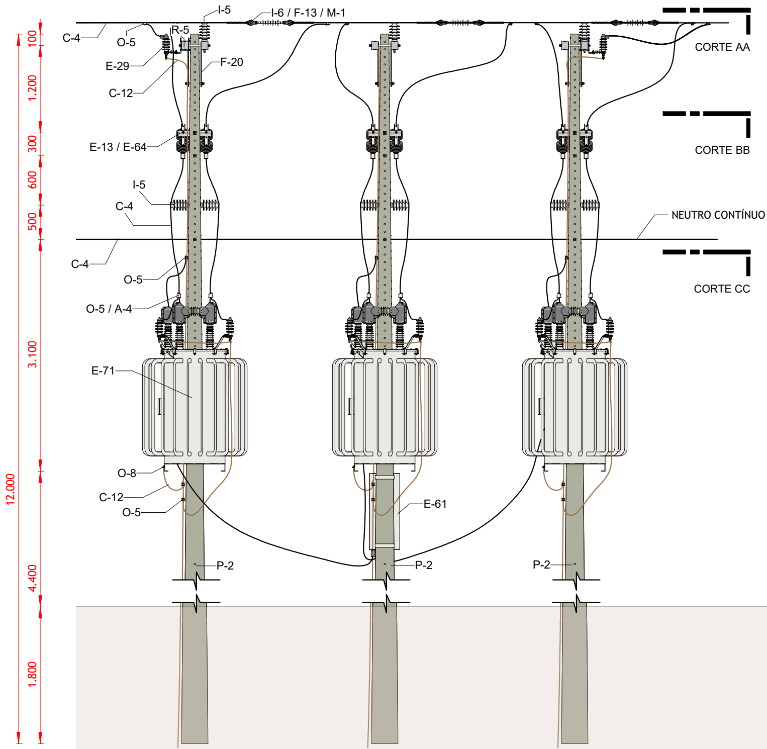
VISTA FRONTAL
