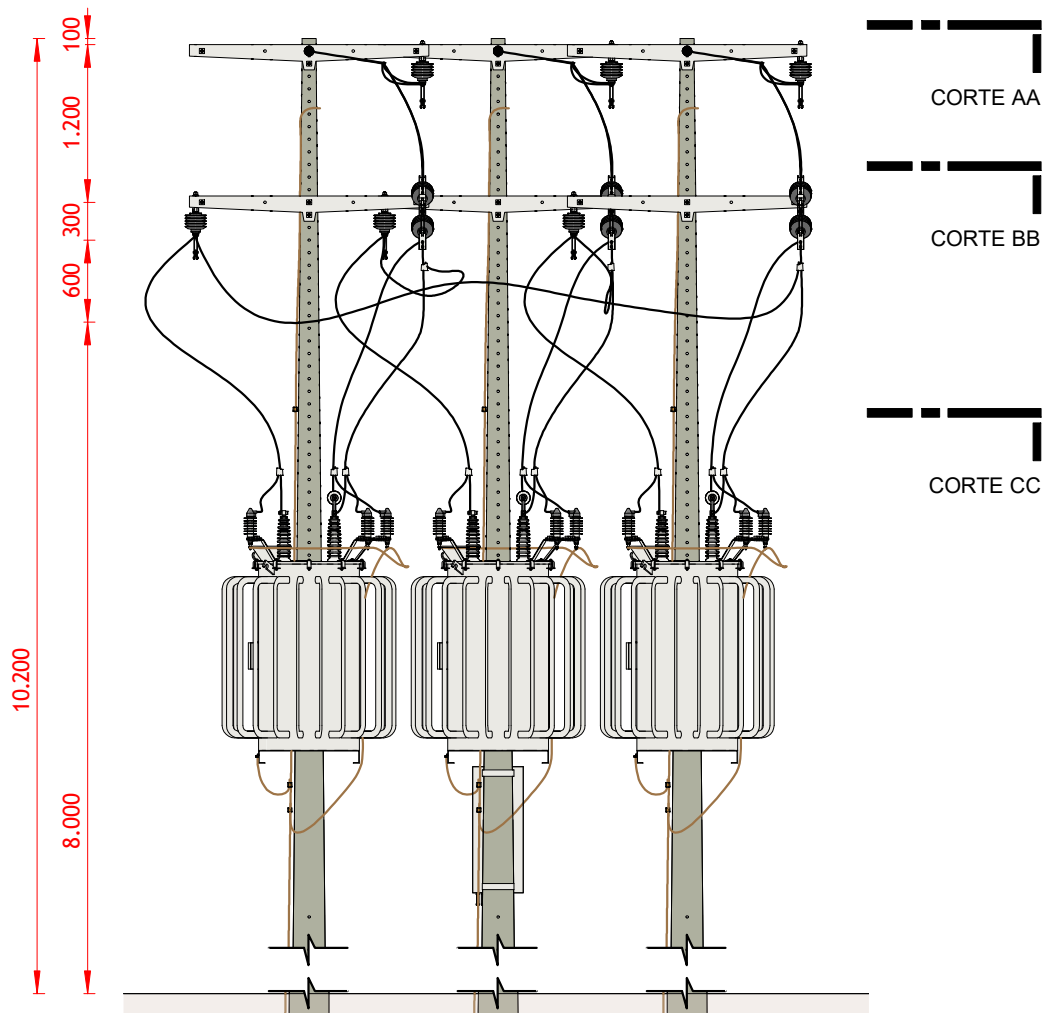
VISTA FRONTAL
