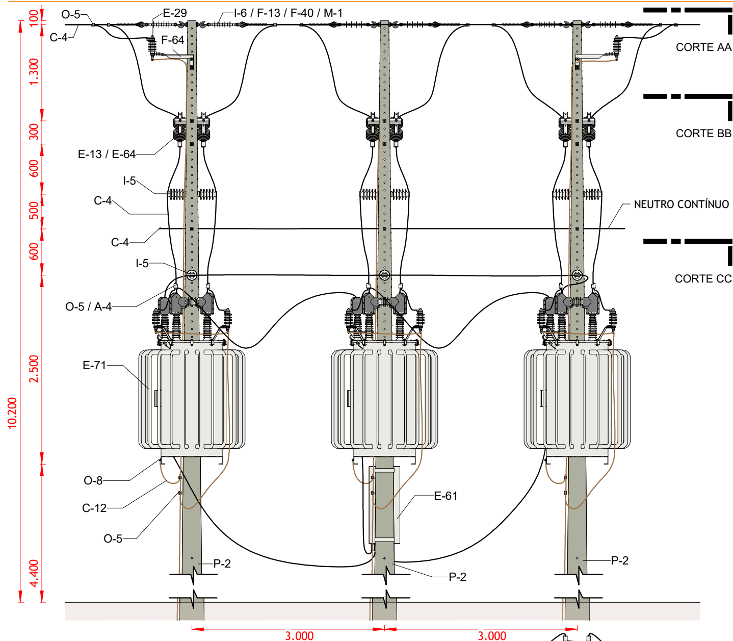
VISTA FRONTAL
