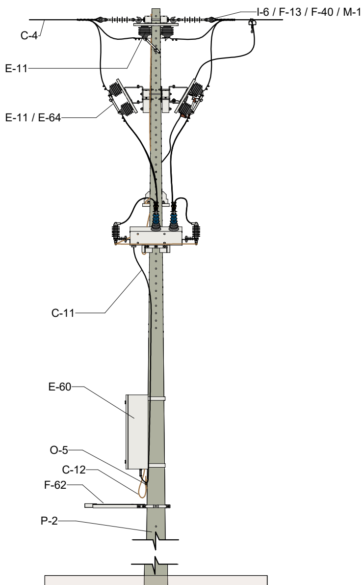
VISTA FRONTAL
