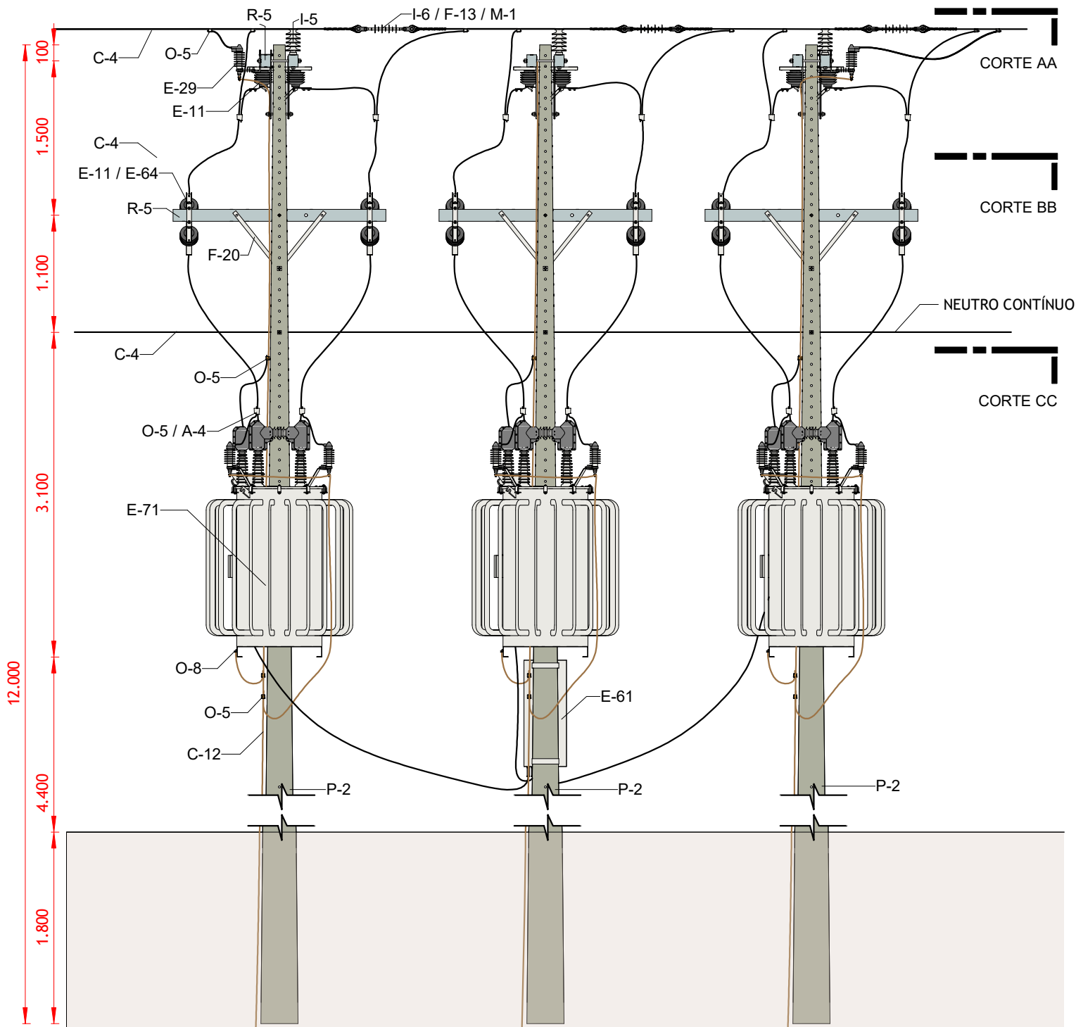
VISTA FRONTAL
