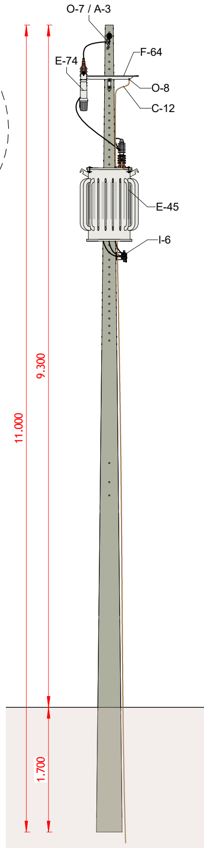
VISTA FRONTAL
