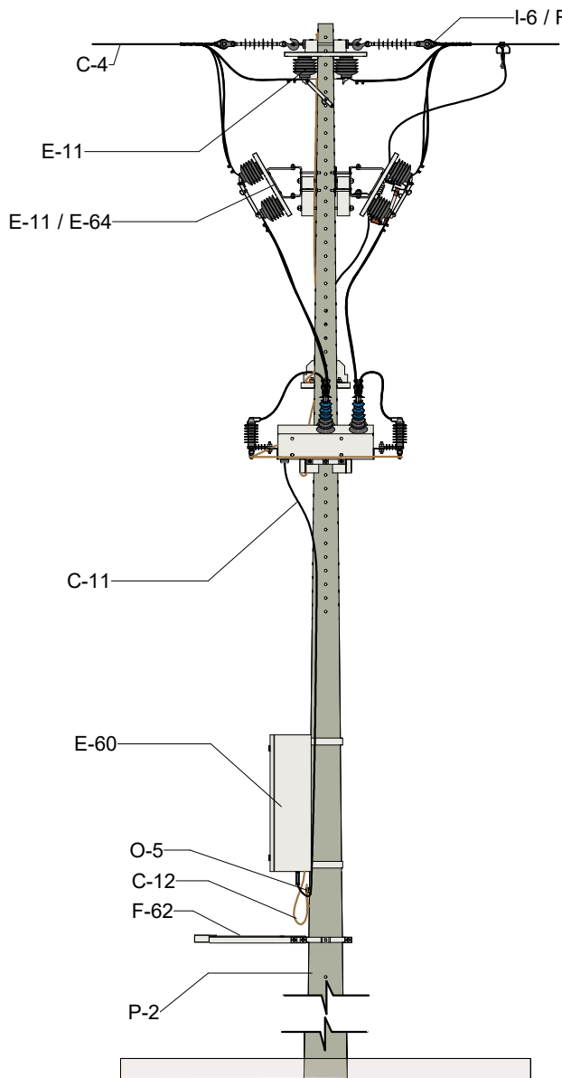
VISTA FRONTAL
