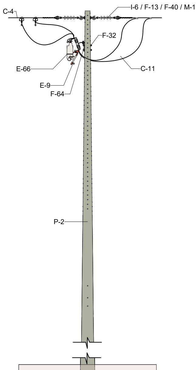
VISTA FRONTAL
