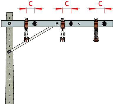
VISTA FRONTAL
