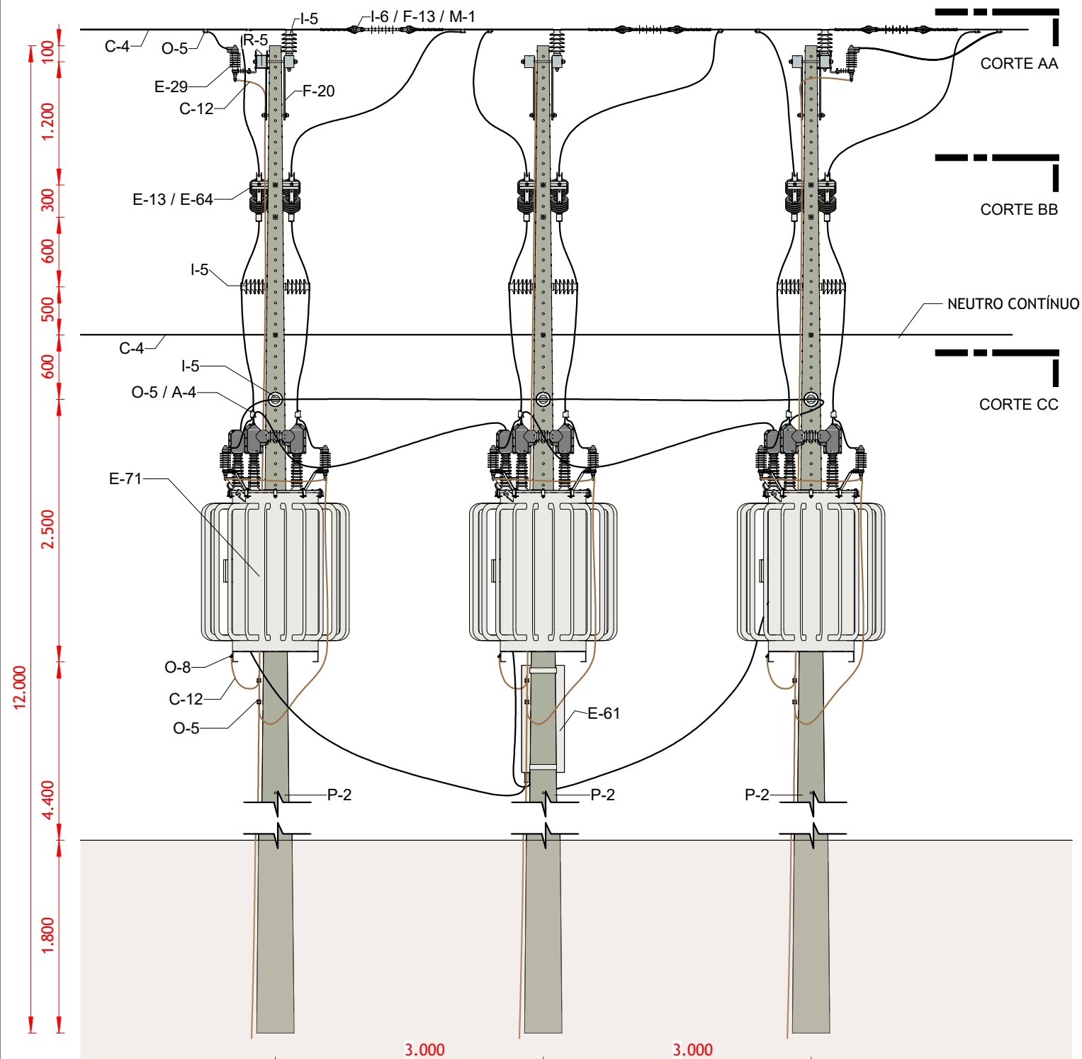
VISTA FRONTAL
