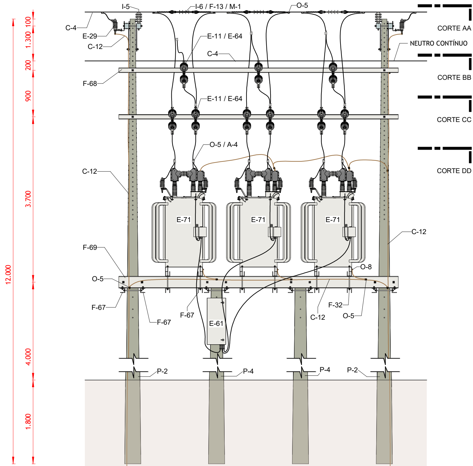
VISTA FRONTAL
