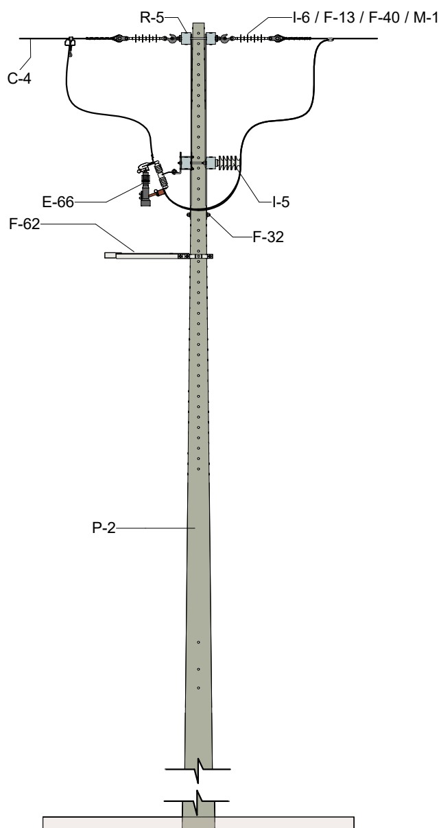
VISTA FRONTAL
