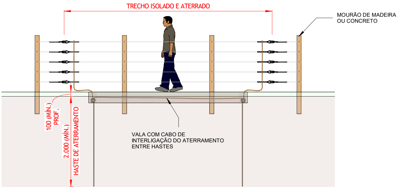
VISTA FRONTAL
