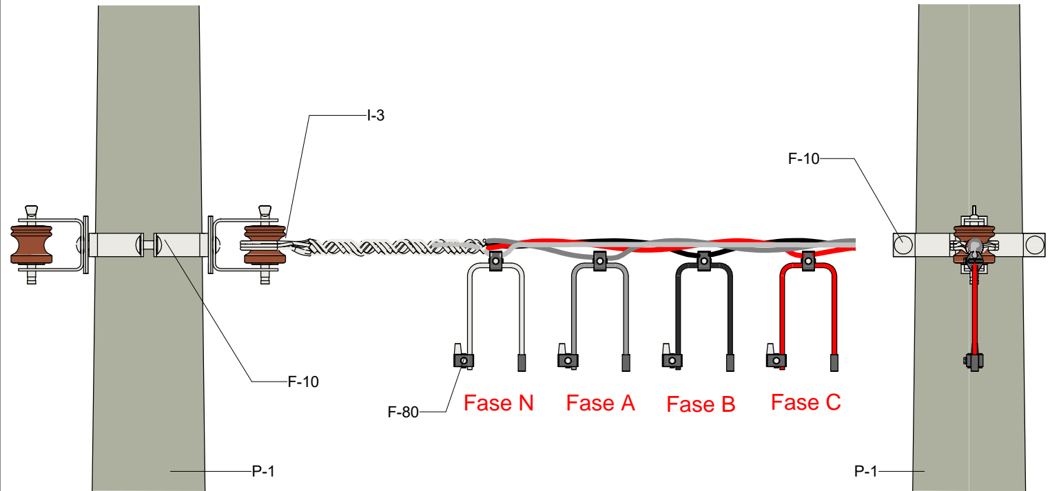
VISTA FRONTAL
