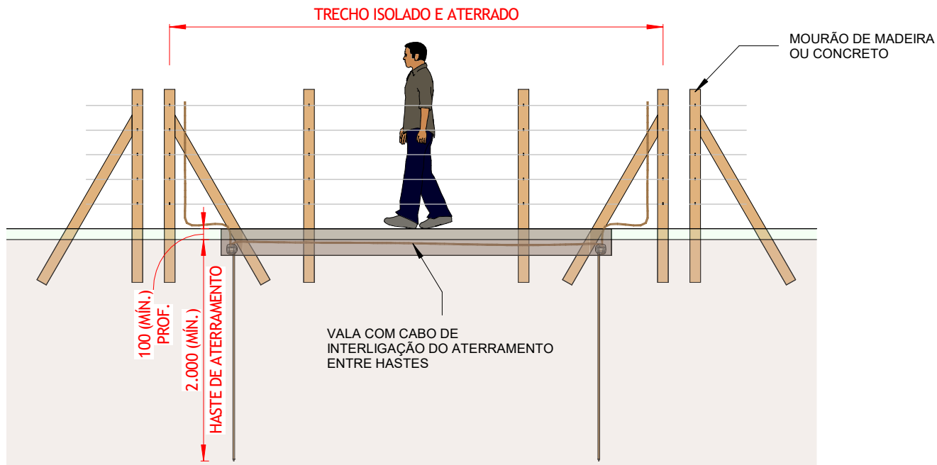
VISTA FRONTAL
