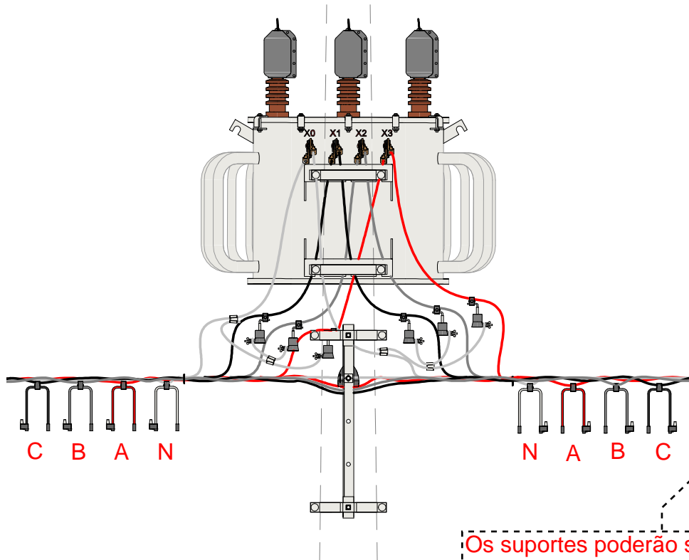
VISTA FRONTAL
