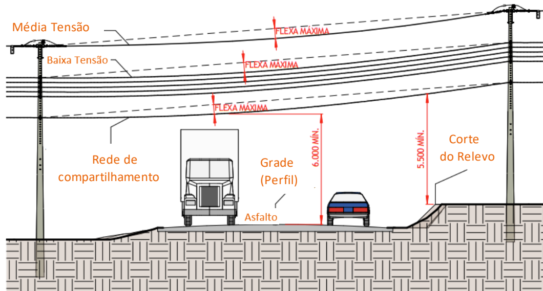
VISTA FRONTAL
