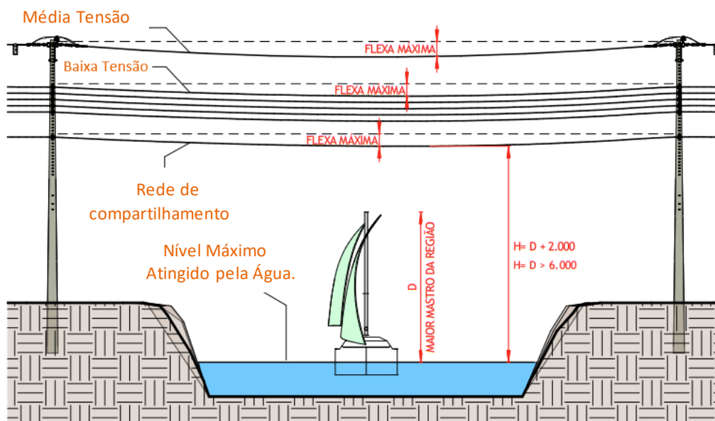
VISTA FRONTAL
