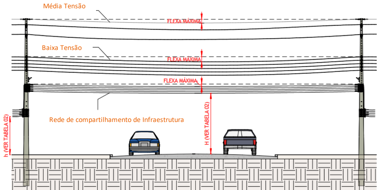
VISTA FRONTAL
